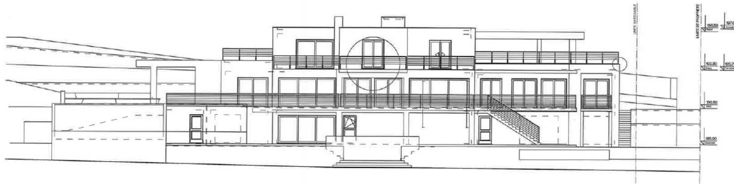
FACADE SUD
